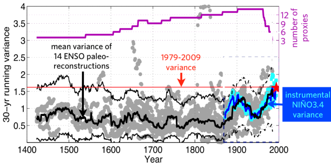
Figure 2. Evolution of ENSO variance in 14 different proxy reconstructions of ENSO over the last 600 years, plotted as the running variance of 10-yr highpass filtered individual reconstructions (grey circles) and as their mean running variance (black line with error envelope). The number of proxy ENSO reconstructions available through time is shown in pink. Also plotted is the evolution of the 10-yr highpass filtered NIÑO3.4 SST variance derived from four different instrumental products (cyan circles), with their mean running variance (blue line). The red star indicates the variance of the 1979-2009 NIÑO3.4 index. Modified after Fig. 7 of McGregor et al. (2013).
