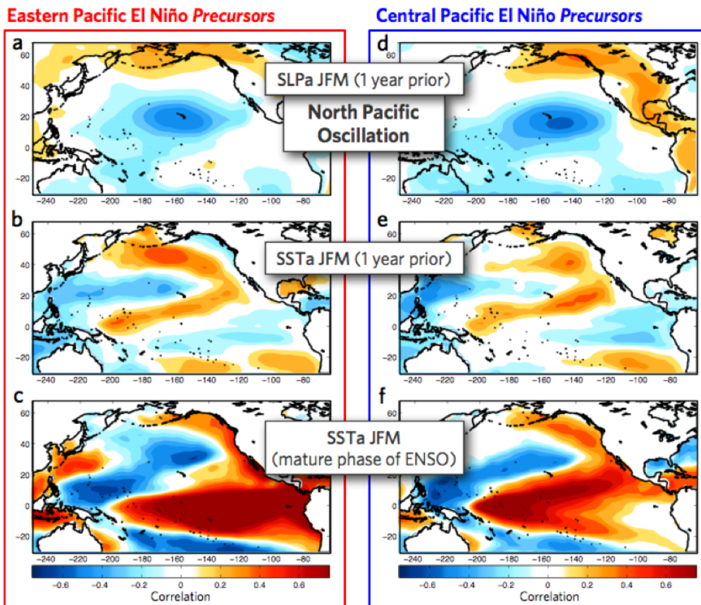
Figure 1. Extra-tropical El Niño precursors in North Pacific SLPa and SSTa. Correlation maps of Niño34 index with SLPa (a) and SSTa (b) in the January/February/March (JFM) one year prior to the mature phase of the eastern Pacific El Niño (c). The same analysis is performed using the central Pacific El Niño index (d,e,f). The maps use the NOAA SSTa and NCEP SLPa. Figure courtesy of Di Lorenzo et al. (2013).
