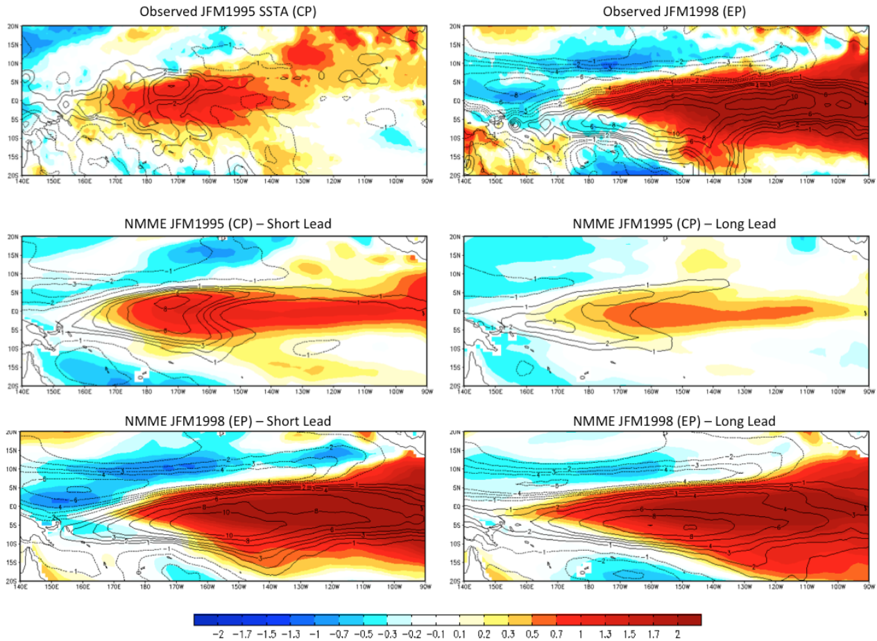
Figure 2. The top row shows SSTA (shaded) and rainfall anomaly (contours) for observational estimates for JFM1995 and JFM1998. Middle row shows the NMME grand ensemble mean JFM1995 SSTA and rainfall anomaly retrospective forecast for short leads (left panel) and long leads (right panel). The bottom row is the same as the middle row except for JFM1998. The rainfall anomaly contour interval is 1 mm day -1 and the SSTA is in °C.
