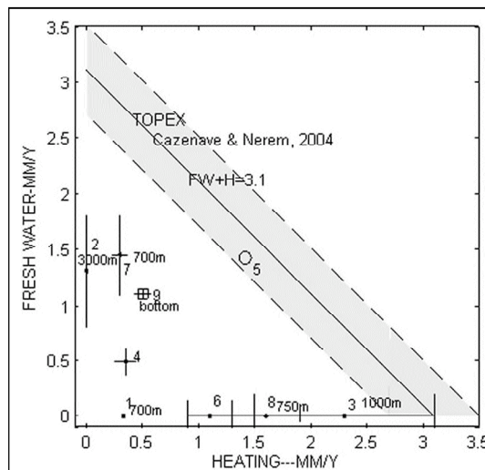
Figure 1. Estimated fresh water and thermal anomaly contributions to global average sea level (Wunsch, Ponte, Heimbach, 2007) including (No. 9) the MIT/AER ECCO-GODAE estimate, 1993-2004. Straight line is the altimetric estimate of Cazenave and Nerem (Rev. Geophys., 2004) which sees only the total change, covering 66S to 66N in latitude. That there is a general lack of consistency among the estimates is a central issue in understanding what is happening with modern sea level rise. Numbers denote the reference paper and the depth to which the investigator carried an integration of temperature or salt anomaly.
