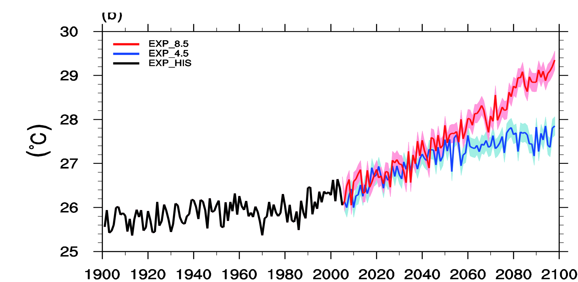
Fig 7. Time series of the annual mean SSTs averaged over the GoM during 1900-2098 obtained from EXP_HIS (black), EXP_4.5 (blue) and EXP_8.5 (red).
