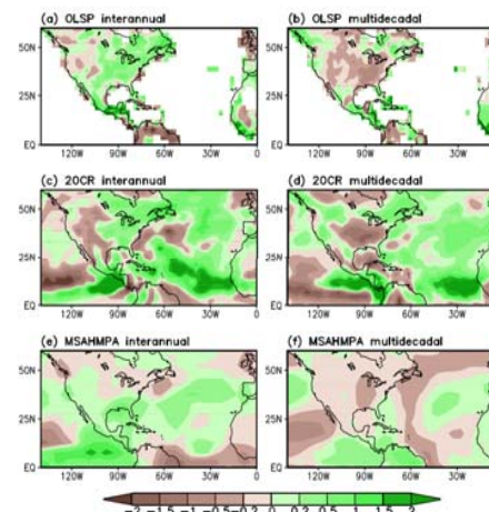
Figure 2. (left) Regression of the precipitation data from (a) OLSLP, (c) 20CR and (e) MSAHMPA onto interannual band AWPTI. (right) Regression of the precipitation data from (b) OLSLP, (d) 20CR and (f) MSAHMPA onto AWPTI of decadal-to-multidecadal band
