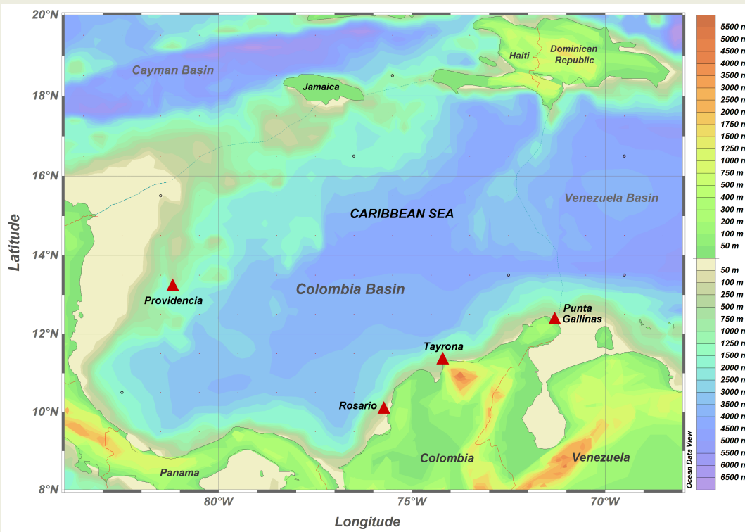
Figure 1. Location of observation points in the Colombian Basin (Caribbean Sea): Providencia, Punta Gallinas, Tayrona and Rosario (above)
