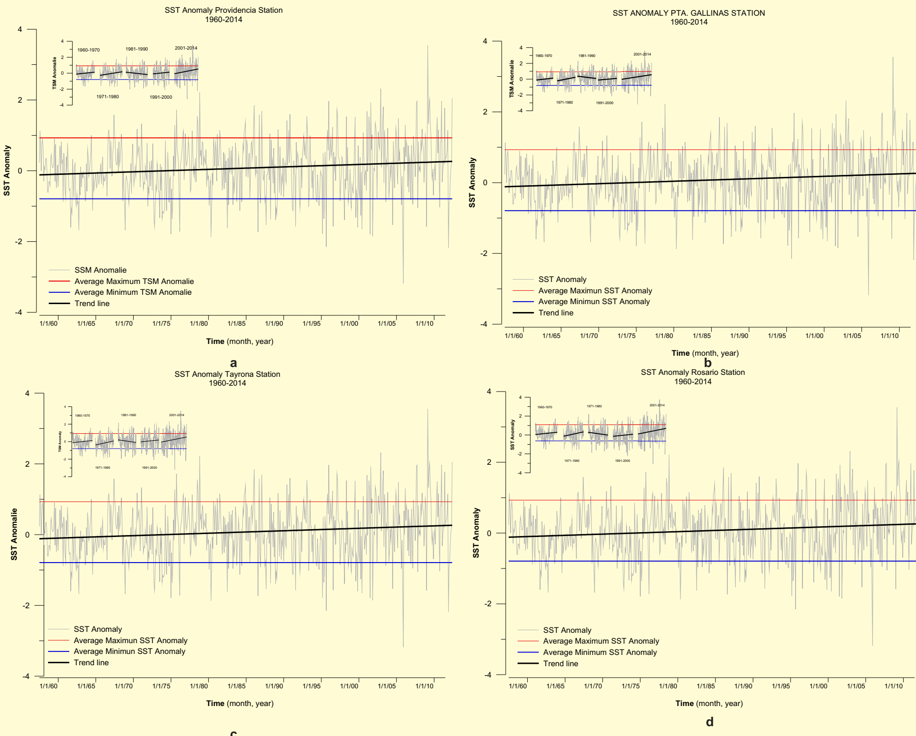
Figure 3. SST anomaly and trend line to 1960-2014 period. For each station analyzed, over each graphic is showed the trend line around decadal period: 1960-1970, 1971-1980, 1981-1990, 1991-2000 and 2001-2014. a) Providencia station b) Punta Gallinas station, c) Tayrona and d) Rosario
